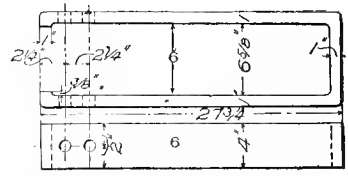
Figs. 20 5-2006. Yoke or Strap-pocket
